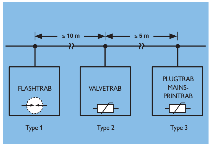
Fig. 4.1-3 Cable as decoupling element
